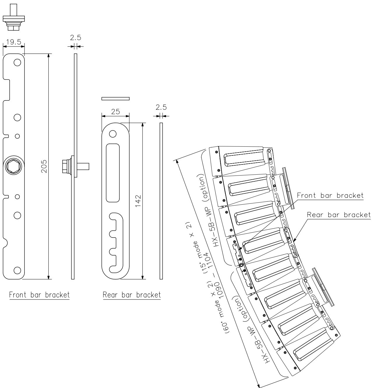
Speaker mounting example (scale: 1/10)
